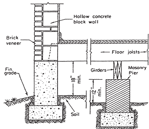
Figure 4-3. Provide adequate clearance between wood and soil.
