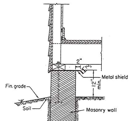
Figure 4-4. Termite shield over uncapped masonry wall.
